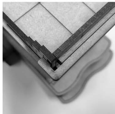
When glued in, you should have a hole like this on both corners to accept acrylic rail signs.
