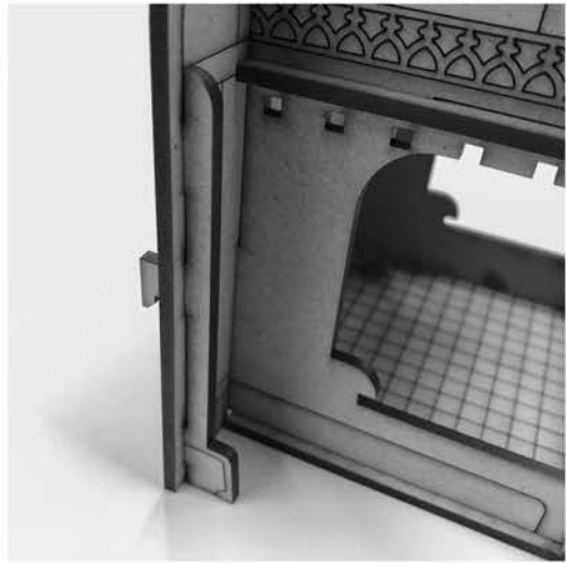
Glue hook rails in on both sides of the back plate.
